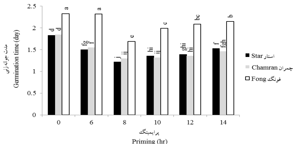
Fig. 1. Mean comparison of seed germination time of three wheat cultivars in interaction effect of seed priming ×cultivar treatments
