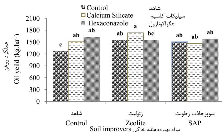
Fig. 2. Interaction effect of soil and plant improvers on oil yield in Tehran ( P \leq 0.05 ).
