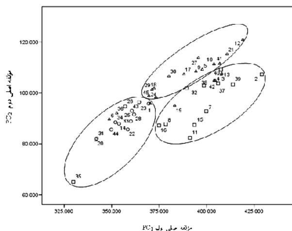
Fig. 2. Biplot of the first and second principal components ( \Delta = first cluster; \square = second cluster; o = third cluster)
