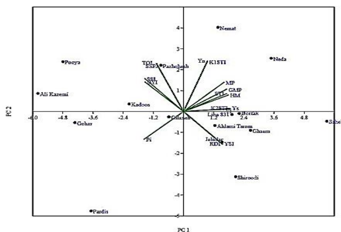
Fig. 3. Biplot of 16 rice genotypes and drought tolerance and susceptible indices based on the first and second principle component
